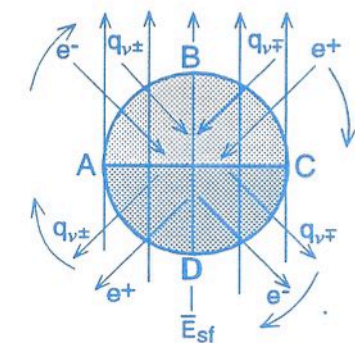
Fig. 3. A - self-emergence starts, decay of heavy elements stops; ABC - self-generation of heavy elements from e^+ , e^- , q_{\nu^+} , q_{\nu^-} charges; C - self generation stops, transmutation starts; CDA - transmutation of heavy elements into the final product ( e^+ , e^- , q_{\nu^+} , q_{\nu^-} ).
