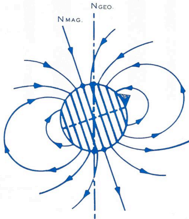
SIMPLIFIED DIAGRAM OF THE MAGNETIC FIELD OF THE EARTH AND RELATIVE LOCATION OF PYRAMID (GIZA)
